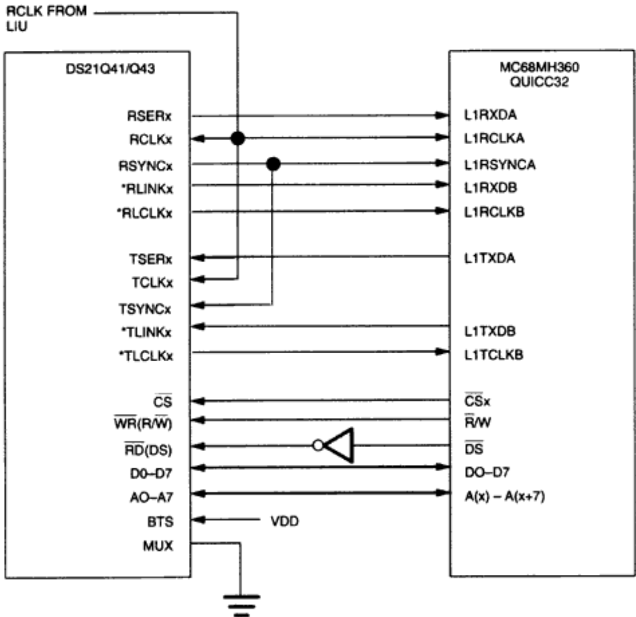
Figure 1. Quad Framer - QUICC32 Interconnections
